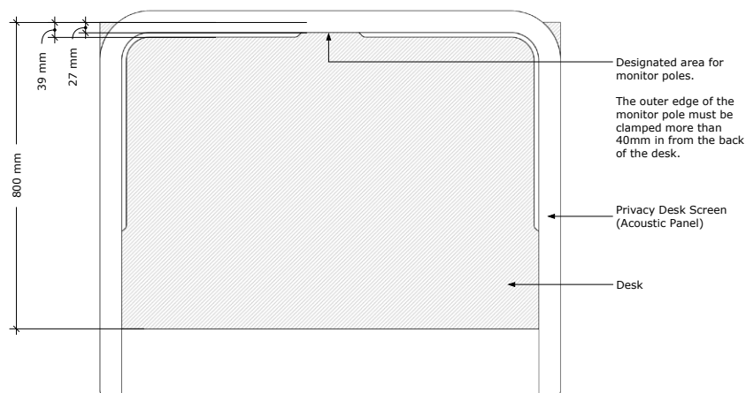
Top View Scale 1:10 @ A3
