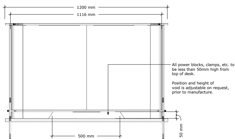
Front View Scale 1:10 @ A3
